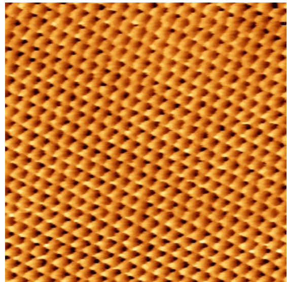
Atomic Resolution on HOPG, LFM. 3nm scan. NO filtering in Fourier space.
