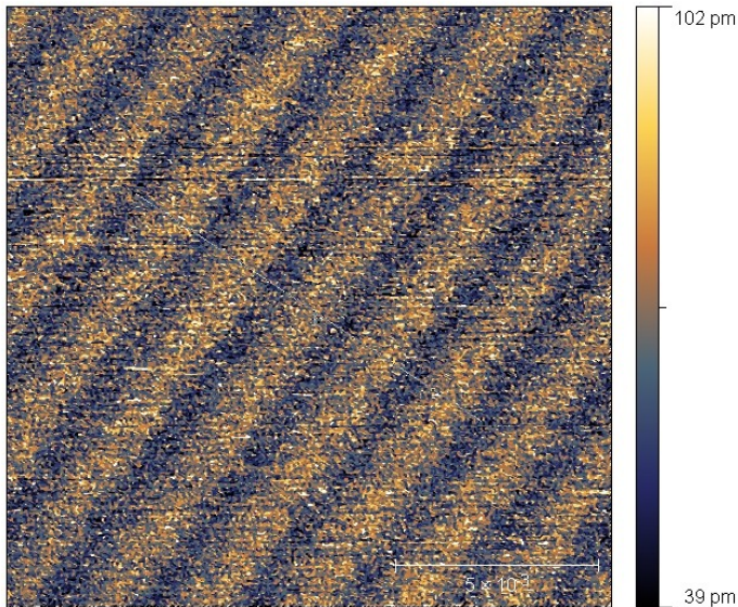
14nm topography scan of C 18 H 38 on HOPG.
