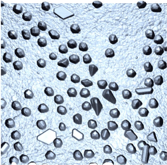
130 nm Ag nanoparticles immobilized on the metal surface
