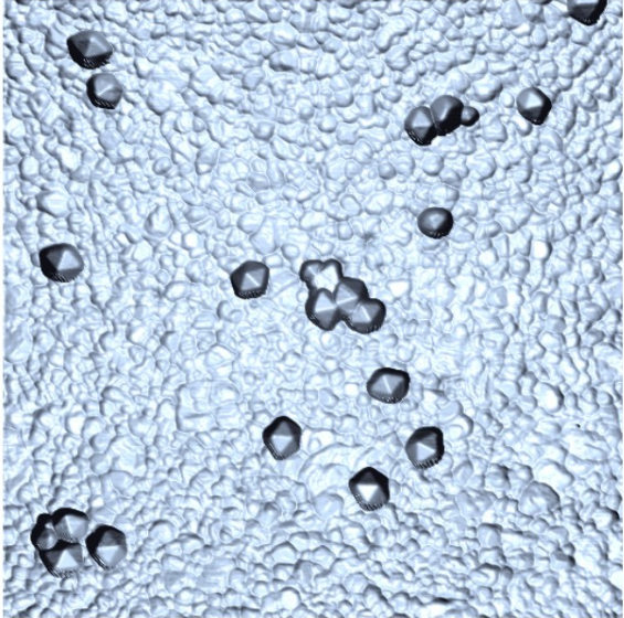
120 nm decahedra immobilized on the metal surface
