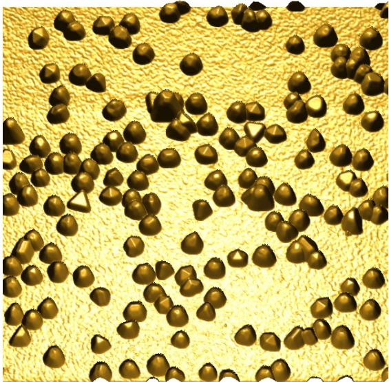
150 nm Au nanoparticles immobilized on the metal surface
